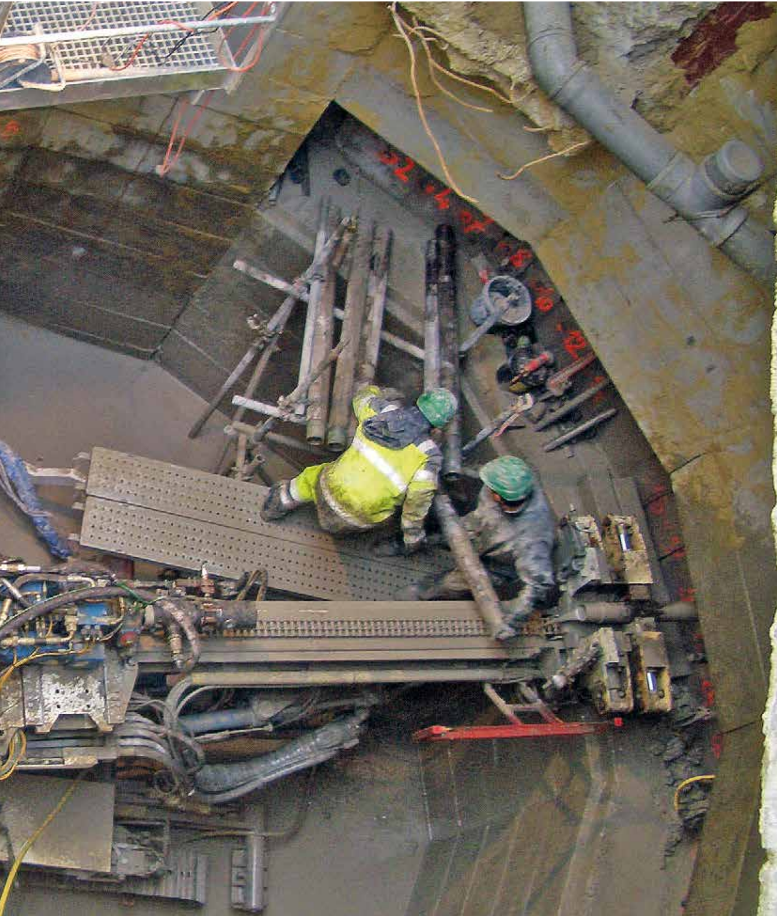
Tunnel Schumann Josaphat (Belgium) Compensation Grouting
